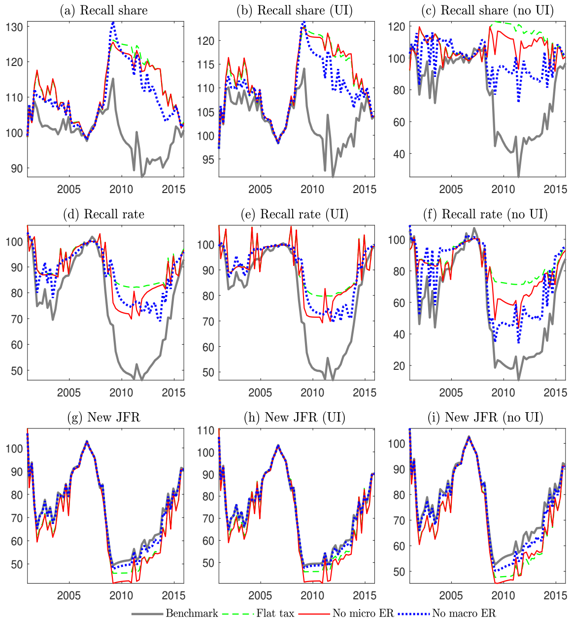
Figure 9: Counterfactual simulations
