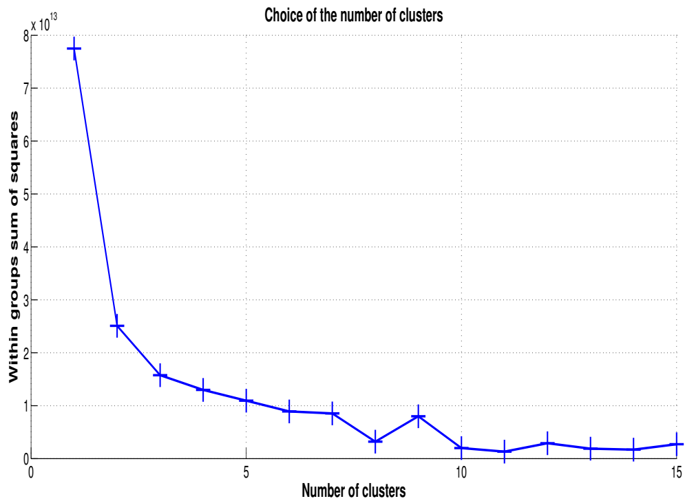
Figure 3: Within groups sum of squares
