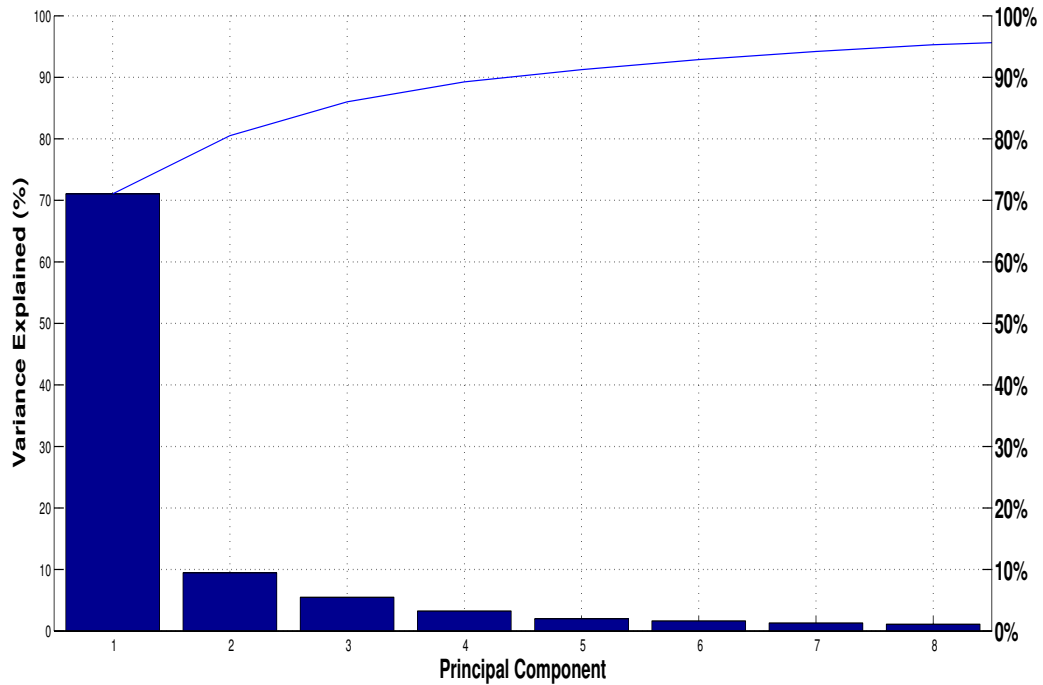
Figure 1: Explained variance for the components obtained via Principal Component Analysis
