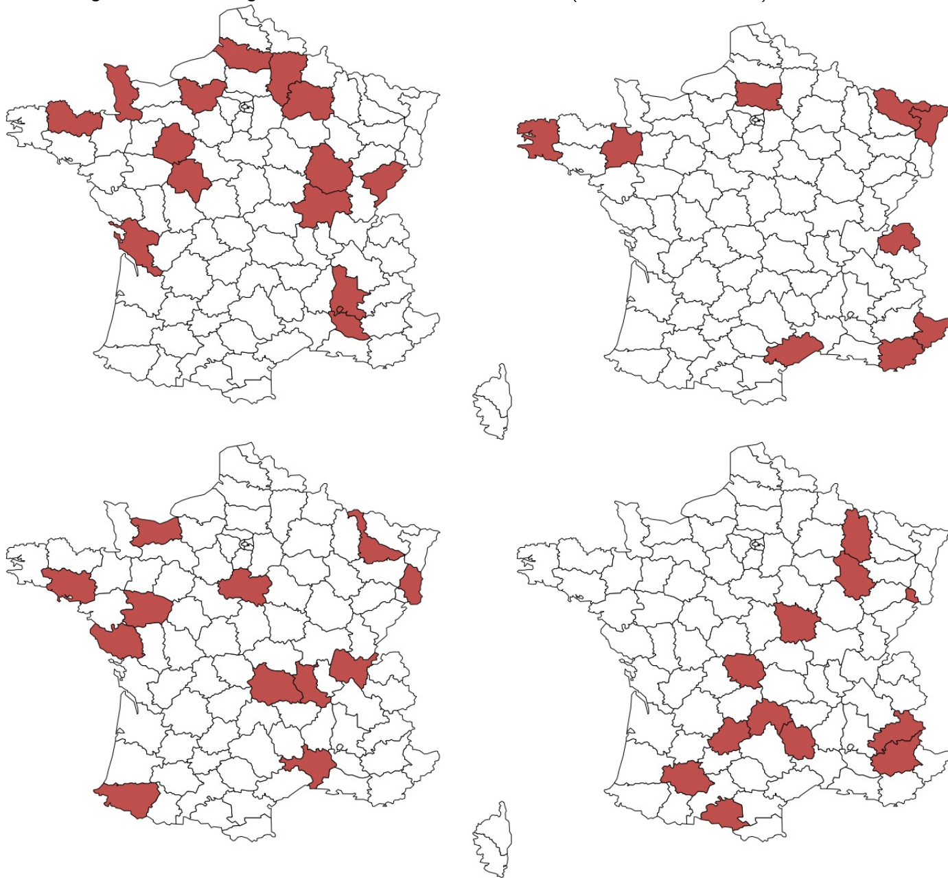
Figure 8: Cluster segmentation for K = 8 for each cluster (ordered Cluster 5 to 8)
