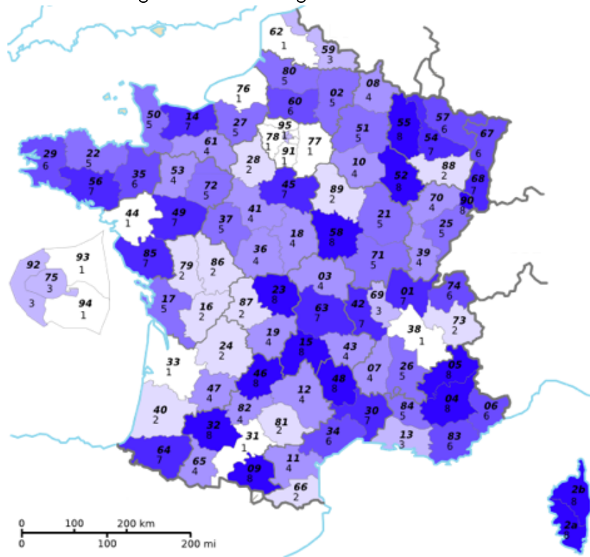
Figure 5: Cluster segmentation for K = 8
