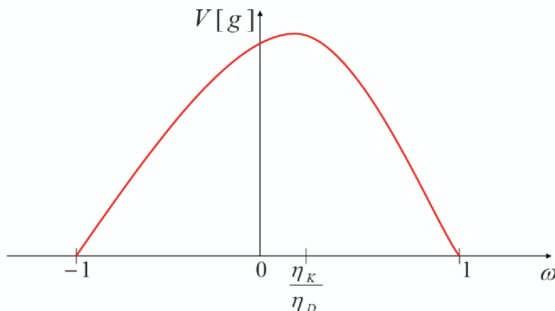
Figure 1: Variance of Growth Rate \mathbf{V}[g] against Risks Correlation \omega Case (ii) of Proposition 3.3
