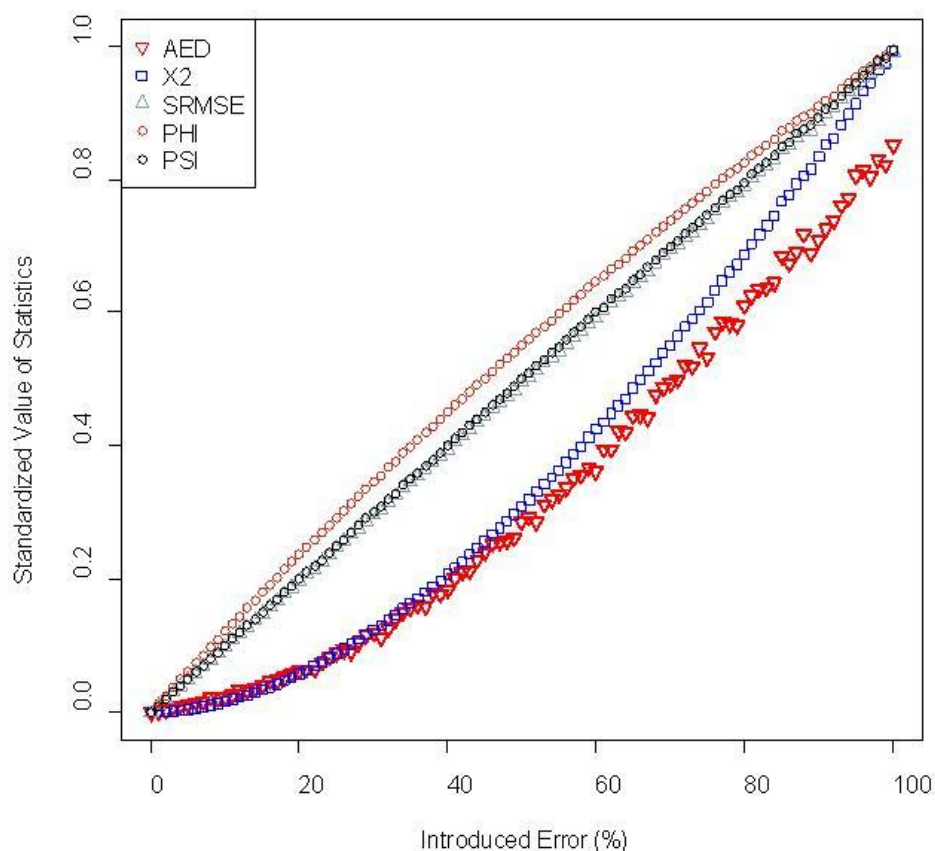
Figure 5: Error sensitivity of five Goodness-of-fit statistics
