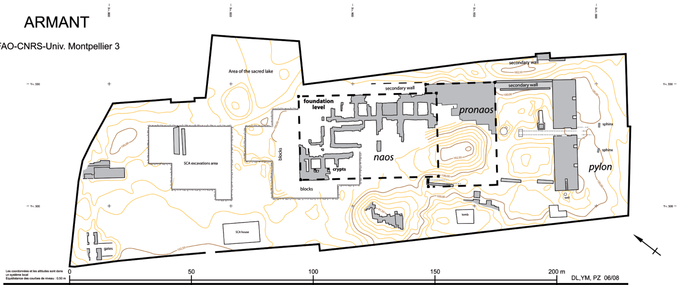
General plan of the temple area at Armant. Plan © IFAO-CNRS/Damien Laisney, Yassin Mohammed and Pierre Zignani
