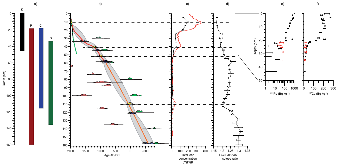
Fig. 2. (a) Cores used in this study. (b) Age model established by the OxCal program when including six radiocarbon dates based on three large ( > 2 mg) macrofossils (dark blue) and three small ( < 2 mg) macrofossils (light blue), a CRS-model based on nine ^{210}\text{Pb} samples (black dots above 15 cm), and four lead pollution markers (yellow, Brännvall et al., 2001). Seven radiocarbon dates based on small macrofossils (red), eight bulk radiocarbon dates (green) and all ^{210}\text{Pb} samples below 15 cm were excluded when constructing the model. Two polynomial functions, one above (red line) and one below 60 cm (orange line), with a polynomial order of seven and two, respectively, were fitted to the midpoints of the calibrated 2\sigma intervals (grey) provided by OxCal and used to calculate ages for the sequence at 0.5 cm intervals. Green line represents the age/depth model used in Fredh et al. (2012). (c) Total lead concentrations measured using Quadrapole ICP-MS (black line) and XRF (red line), respectively. (d) Lead 206/207 ratio. (e, f) Unsupported ^{210}\text{Pb} and ^{137}\text{Cs} concentrations measured on core K (black) and core P (red).
