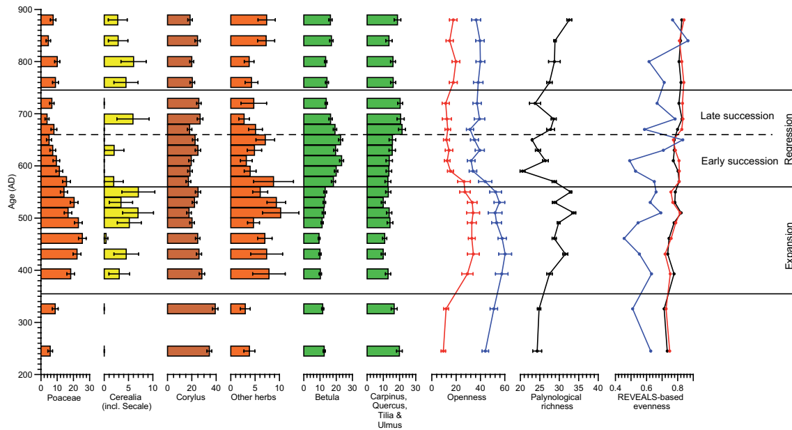
Fig. 5. Regional vegetation cover for selected taxa/taxa groups, openness, palynological richness and REVEALS-based evenness at the transition from expansion to regression AD 350 to 750. Openness was estimated both including and excluding shrubs ( Juniperus and Corylus ) shown by blue and red lines, respectively. REVEALS-based evenness was calculated for all 26 reconstructed taxa (black line), but also for trees (red line) and herbs (blue line) separately. The transition was divided into one expansion and two regression phases.
