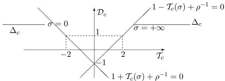
Figure 2: Oscillating/monotone convergence of closed-economy equilibrium.
