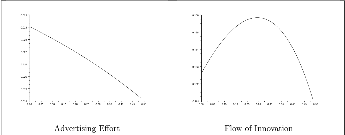
Figure 4: Competition and average sectoral advertising effort and flow of innovation: simulation results.
