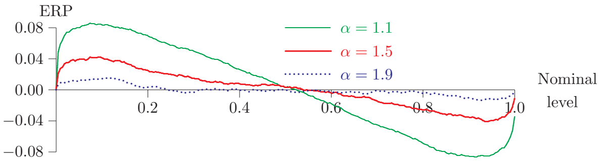
Figure 11: P value discrepancy plots, \hat{\alpha}_{Hill} , \hat{\beta}_{Hill} , stable law
