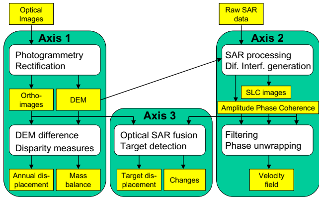
Figure 1: Flowchart of the processing steps to extract information from optical and SAR data to monitor glacier evolution.
