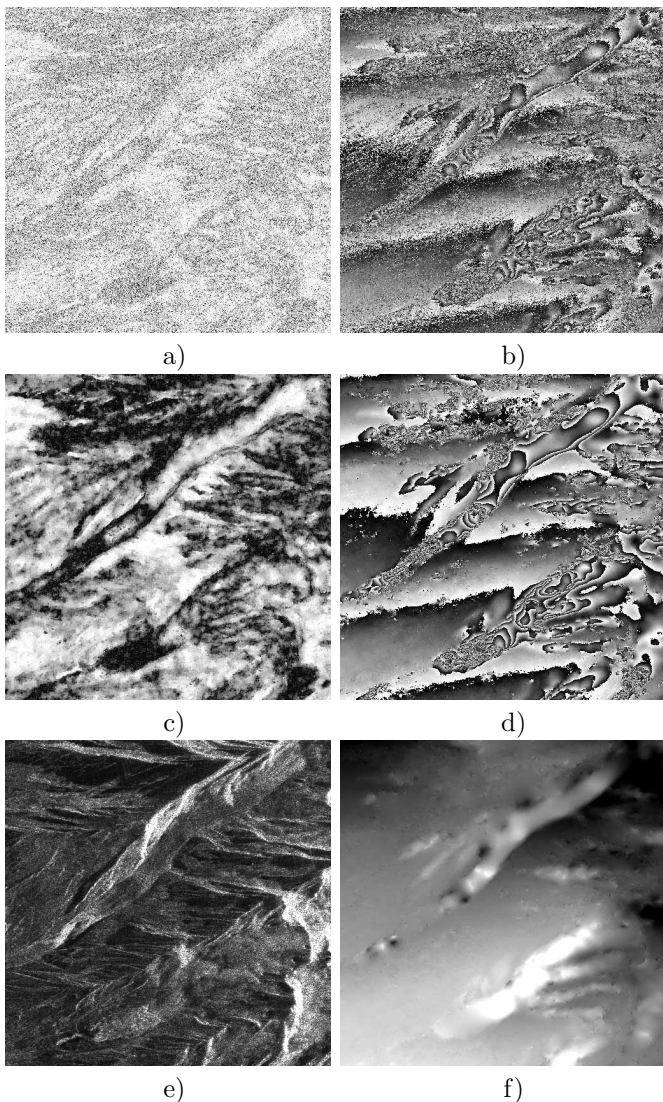
Figure 4: March 10-11 1996 Interferogram over Argentière glacier: a) coherence, b) phase e) amplitude after initial multi-look; c) coherence d) phase filtered by adaptive neighborhood technique, f) unwrapped phase.
