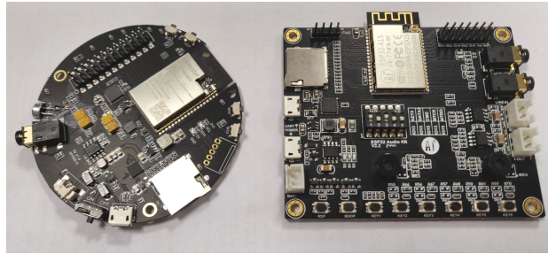
Figure 1. ESP32-based audio Processing boards (the TTGO TAudio on the left and the AI-Thinker Audio Dev Kit on the right).
