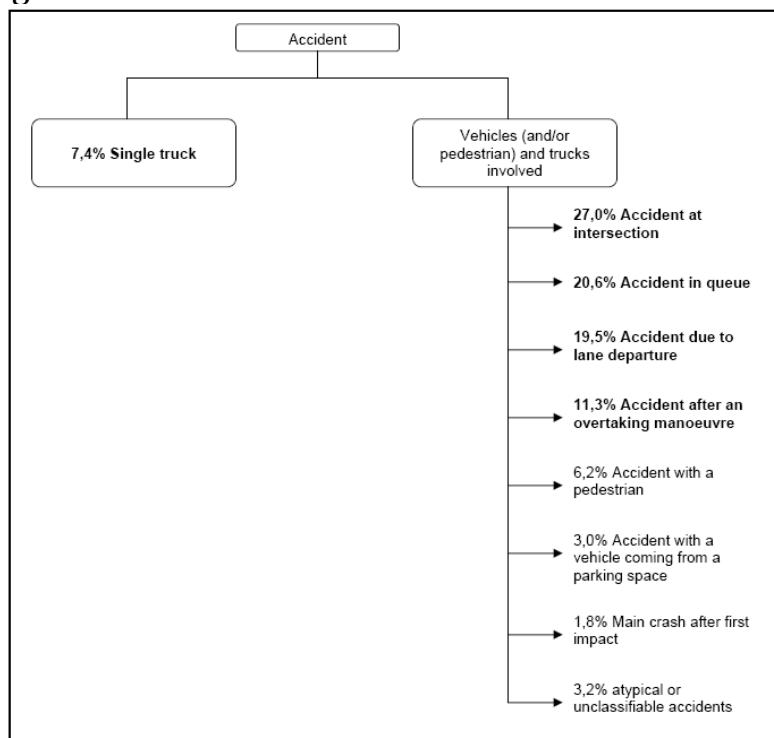
Figure 5.C.3.-Accident configurations.
