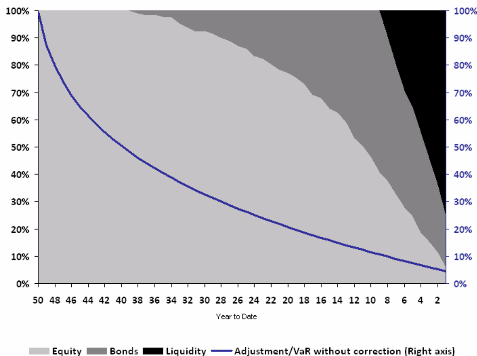
Figure 4 Time-horizon Safety First Allocations in the Main Asset Classes and Historical VaR Errors
