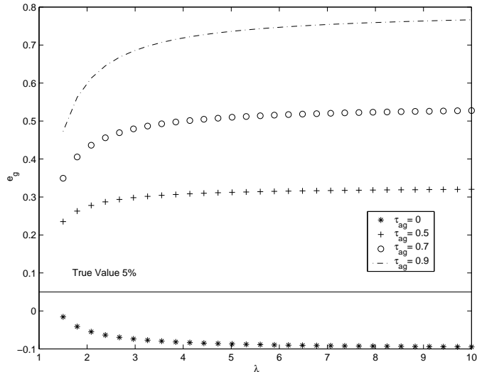
Figure 2: Asymptotic Distribution of \hat{e}_g under OCSR
