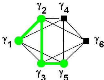
Figure 4: Illustration of a walk in a graph
