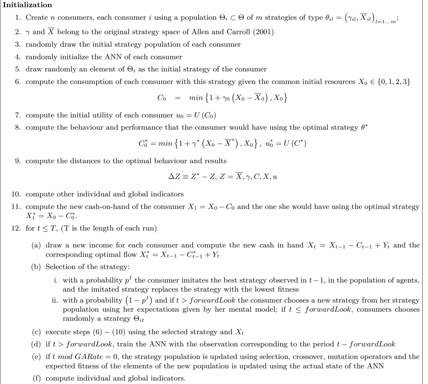
Figure 4: Pseudo code of the learning with expectations model
