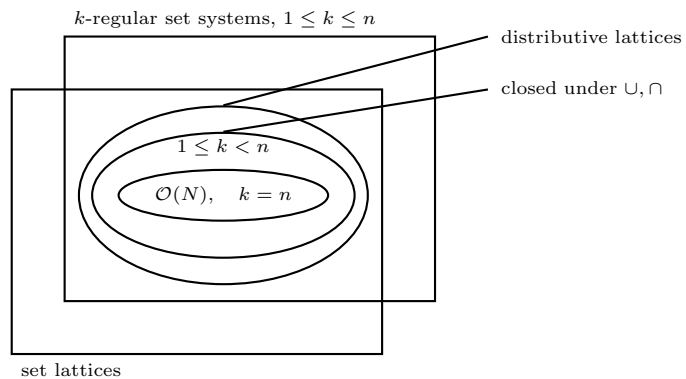
Fig. 3.2. Set lattices and k -regular set systems
