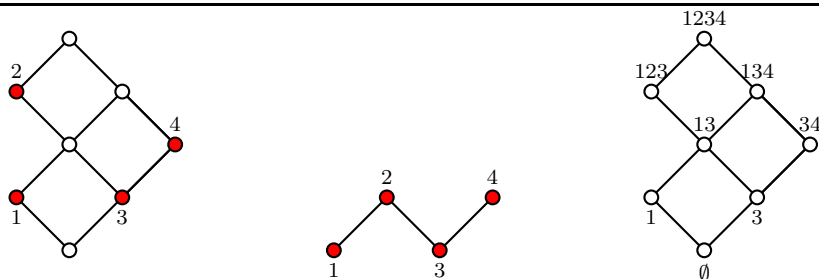
Fig. 2.1. Left: a distributive lattice L . Join-irreducible elements are those in grey. Middle: the poset \mathcal{J}(L) of join-irreducible elements. Right: the set \mathcal{O}(\mathcal{J}(L)) of all downsets of \mathcal{J}(L) ordered by inclusion, which is isomorphic to L
