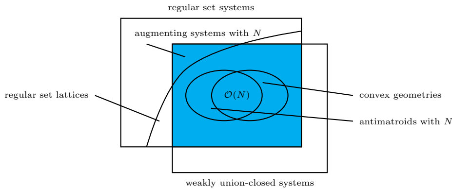
Fig. 3.4. Regular set systems and weakly union-closed systems
