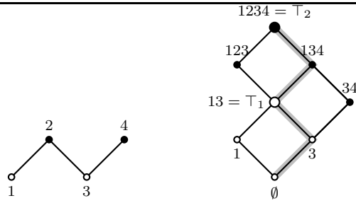
Fig. 5.2. The poset (N, \leq) (left) and the generated lattice \mathcal{O}(N) (right). Level sets on (N, \leq) are Q_1 = \{1, 3\} and Q_2 = \{2, 4\} , inducing level sets S_1 = \{1, 3, 13\} and S_2 = \{34, 123, 134, 1234\} in \mathcal{O}(N) . A restricted maximal chain is drawn in grey.
