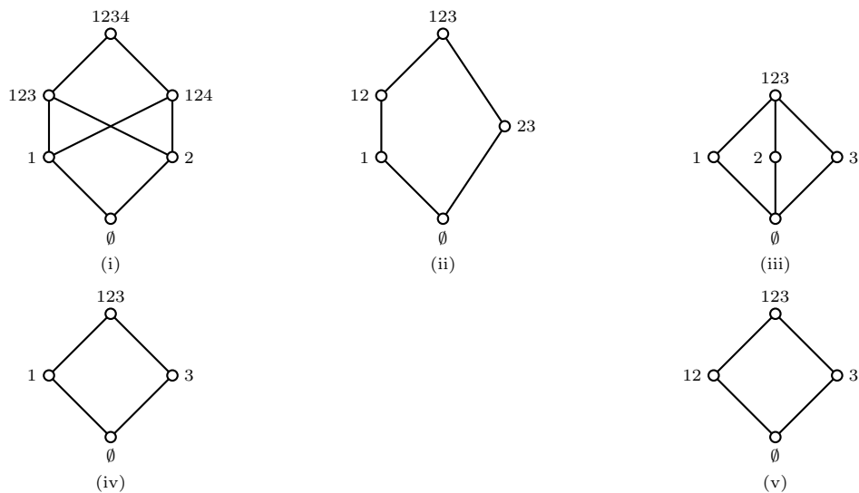
Fig. 3.3. (i) k -regular but not a lattice; (ii) lattice but not k -regular; (iii) k -regular lattice but not distributive; (iv) distributive lattice but not closed under \cup ; (v) closed under \cup, \cap but not isomorphic to \mathcal{O}(N)
