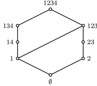
Fig. 3.1. A set system satisfying one-point extension and accessibility, but which is not k -regular
