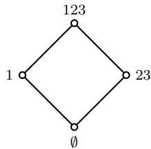
Fig. 5.1. Example of a degenerate 2-regular set system with 3 players
