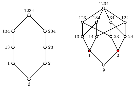
Fig. 3.5. Left: regular set lattice but not weakly union-closed. Right: regular and weakly union-closed but not a lattice, since 1 and 2 have no supremum
