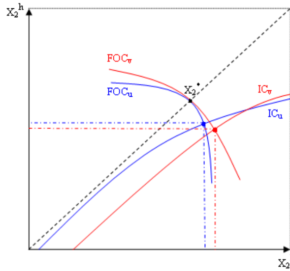
Figure 5: Comparative foresight in the case of CRRA preferences
