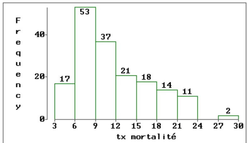
Histogramme
