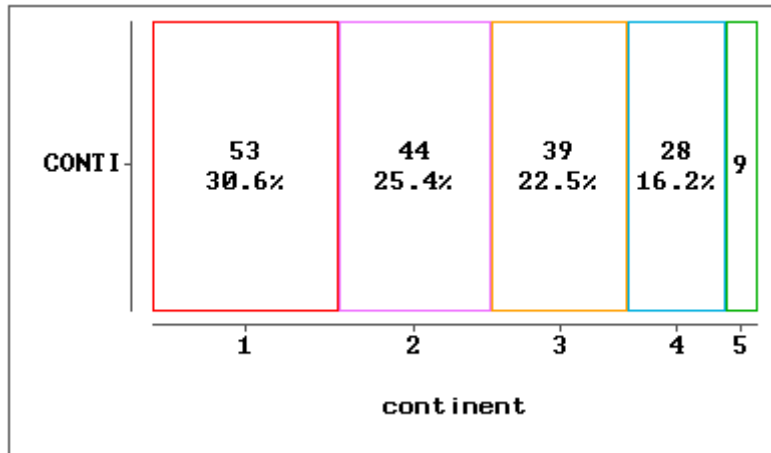
Mosaic Plot
