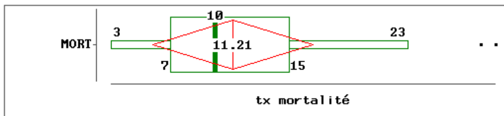
Box Plot
