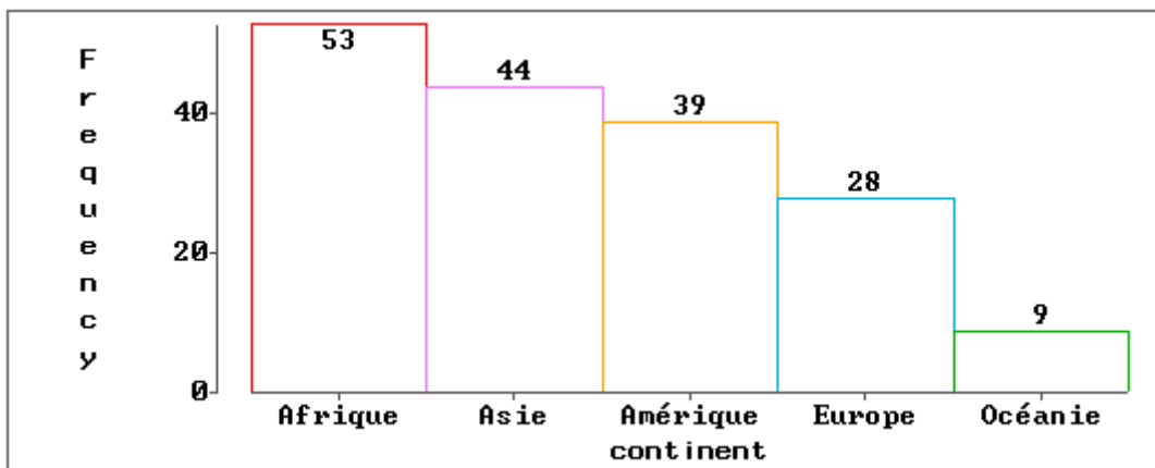
Bar Chart
