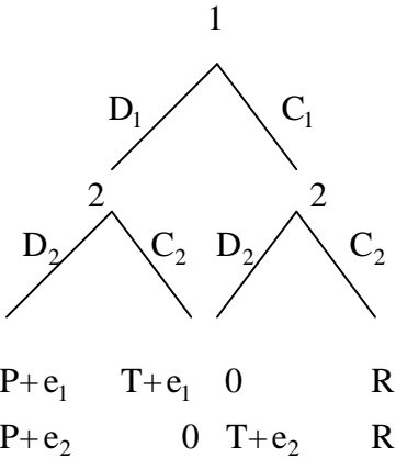
Figure (3). Kantian SPD
