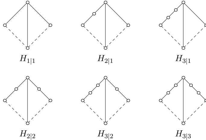
Figure 1: Some s-graphs
