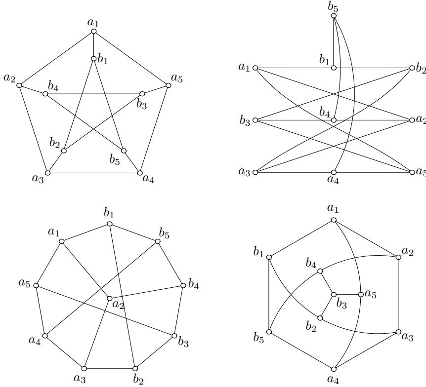
Figure 3: Four ways to draw the Petersen graph
