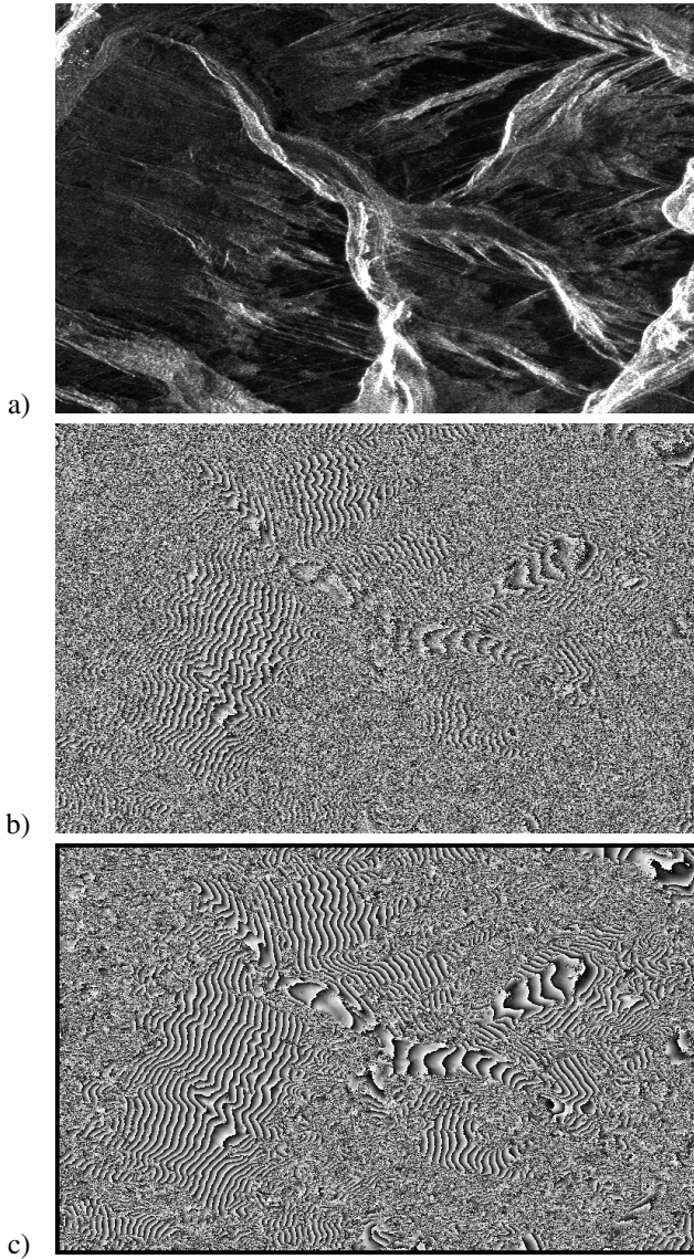
Fig. 1. TANDER ERS 1/2 interferogram: a) SAR amplitude, b) original phase, c) ADAN filtered phase.
