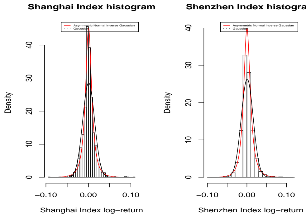
Fig. 2. Asymmetric NIG fitting for log-returns of Shanghai Stock Composite Index and Shenzhen Stock Composite Index
