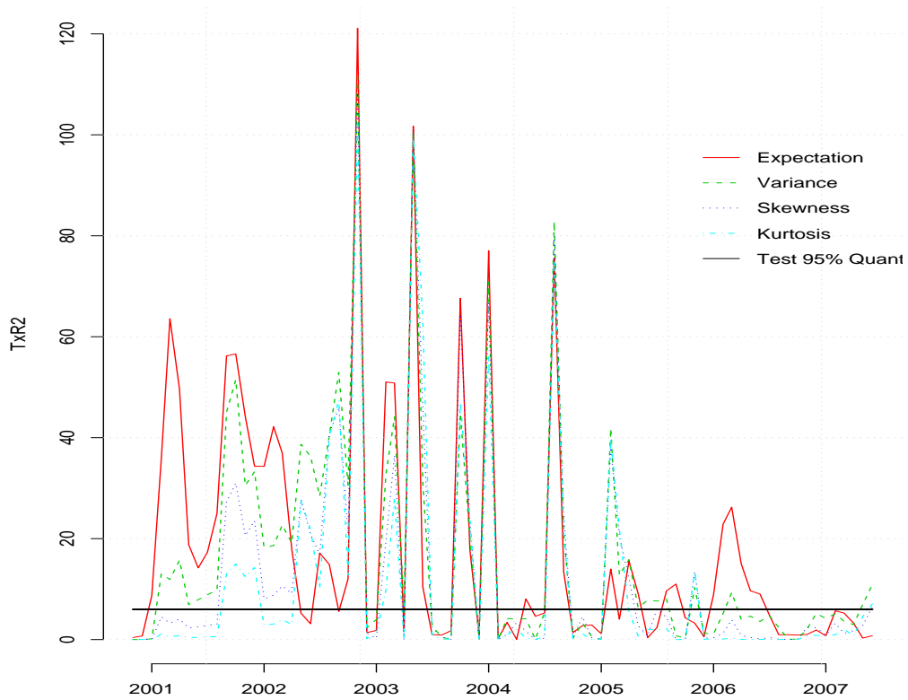
Figure 6: Engle (1982)'s T \times R^2 test for autoregressive moments.
