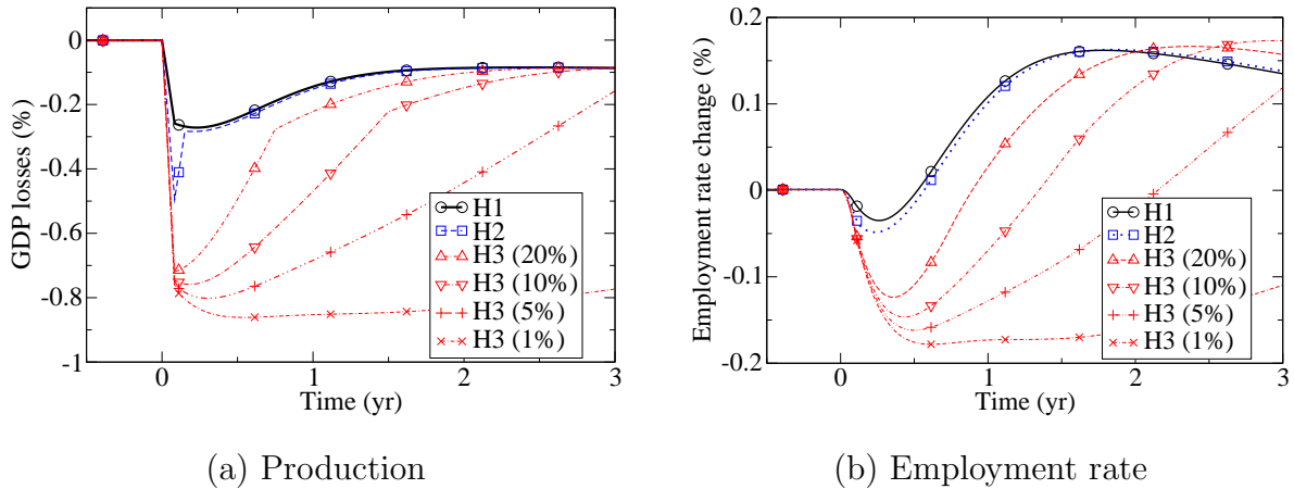
Fig. 5. Production and employment rate pathways, in response to a disaster destroying capital amounting for 3% of GDP, in the classical hypothesis H1 (only the less efficient capital disappears), H2 (capital disappear equally with respect to its efficiency) and H3 (reconstruction investments are limited).
