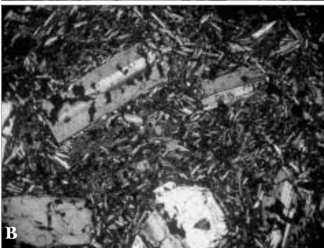
Fig. 5. Doleritic porphyric lava at Wutale East Gully: A, natural light; B, polarized light. Cliché G. Kieffer
