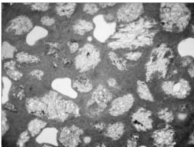
Fig. 26. Gombore II, tuff 2155/58 (sample 2158); microscopic view of vesiculated tuffs in natural light. Cliché G. Kieffer
