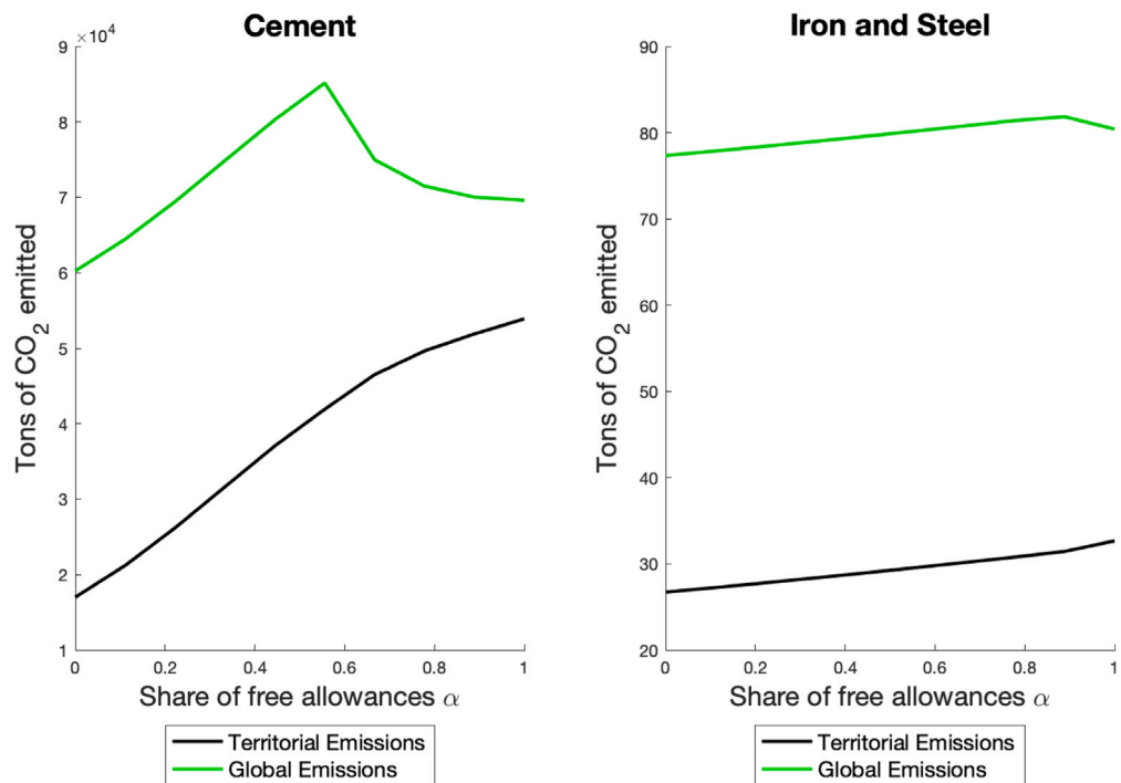
Fig. 6. Emissions with CBAM, with \tau = 162 .
