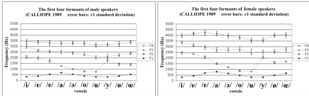
Figure 5 The first 4 formants (in Hertz) of the 10 oral vowels of French pronounced in [pV] and [pV R ] by 10 male (left) and 9 female (right) native speakers of French. Two repetitions per subject (CALLIOPE 1989: 84).
