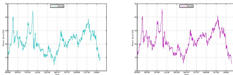
Figure 1 Carbon futures prices of maturities December 2008 (left) and 2009 (right) from April 22, 2005 to January 16, 2009
