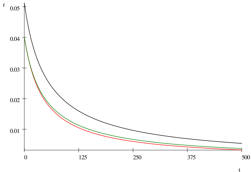
Figure 3: This figure represents the marginal discount rate curve r_t = \frac{\sum_{i=1}^N \frac{w_i \rho_i \exp(-r^i t)}{\sum_{j=1}^N w_j \rho_j \exp(-r^j t)} r^i = \frac{\alpha_1 + 1}{\beta_1 + t} + \frac{\alpha_2}{\beta_2 + t} obtained through our calibration (upper curve) and compares it to the discount rate curve r_t = \frac{\alpha}{\beta + t} of Weitzman (2001) (lower curve). The intermediate curve represents, with our calibration, the unweighted average \sum_{i=1}^N \frac{w_i \exp(-r^i t)}{\sum_{j=1}^N w_j \exp(-r^j t)} r^i = \frac{\alpha_1}{\beta_1 + t} + \frac{\alpha_2}{\beta_2 + t} . It is clear that the difference between our discount rate curve and Weitzman (2001)'s curve mainly results from the fact that, contrarily to the certainty equivalent approach, more impatient experts are more heavily weighted in the equilibrium approach.
