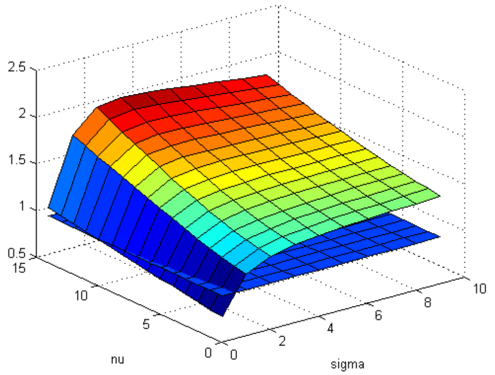
Figure 13: R_0 as a function of \nu and \sigma for \eta = 5.7
