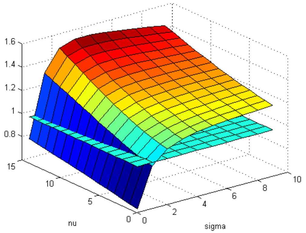
Figure 12: R_0 as a function of \nu and \sigma for \eta = 3.4
