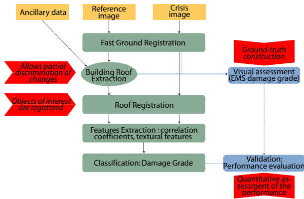
Fig. 1. Block diagram for damage assessment using a pair of panchromatic QuickBird images and ancillary data.
