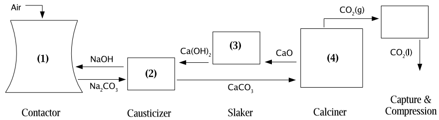
Figure 5: Top level process diagram of an example direct air capture system. Closed chemical loops of \text{NaOH} and \text{CaO} extract \text{CO}_2 from air convert it to a pure, compressed form for sequestration.
